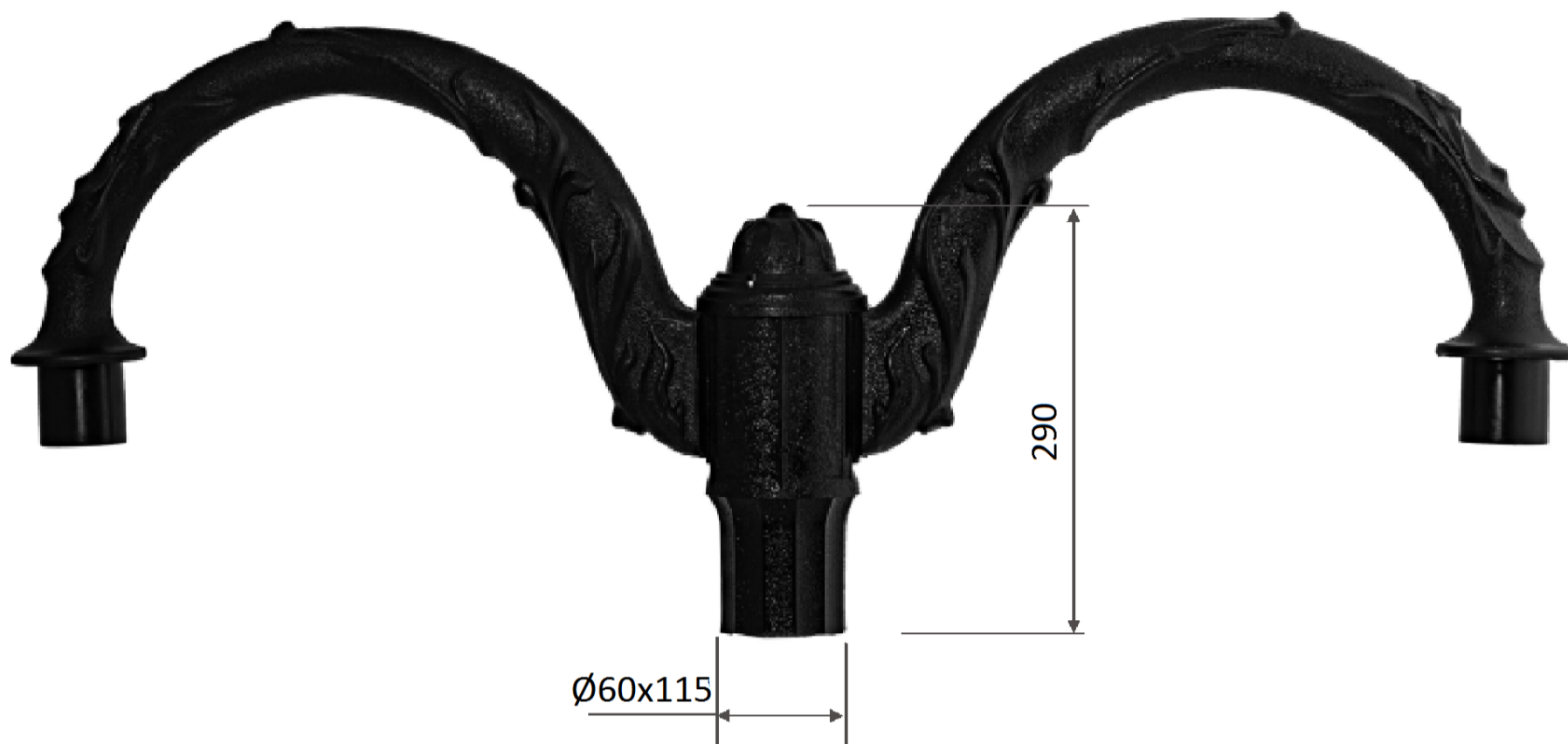
Arm system „2” downwards
