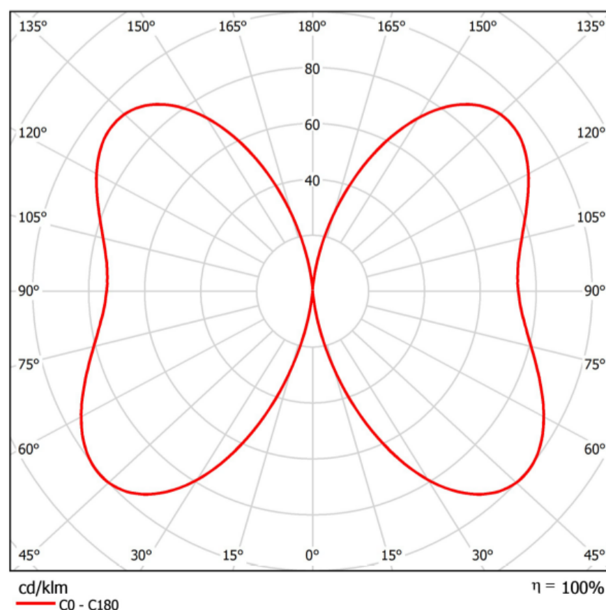
Distribution curve KARIN DECOR 4800 LED
